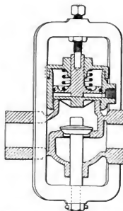
Fig. 3338. Pneumatic Blow-off Cock, Yoke Type.
